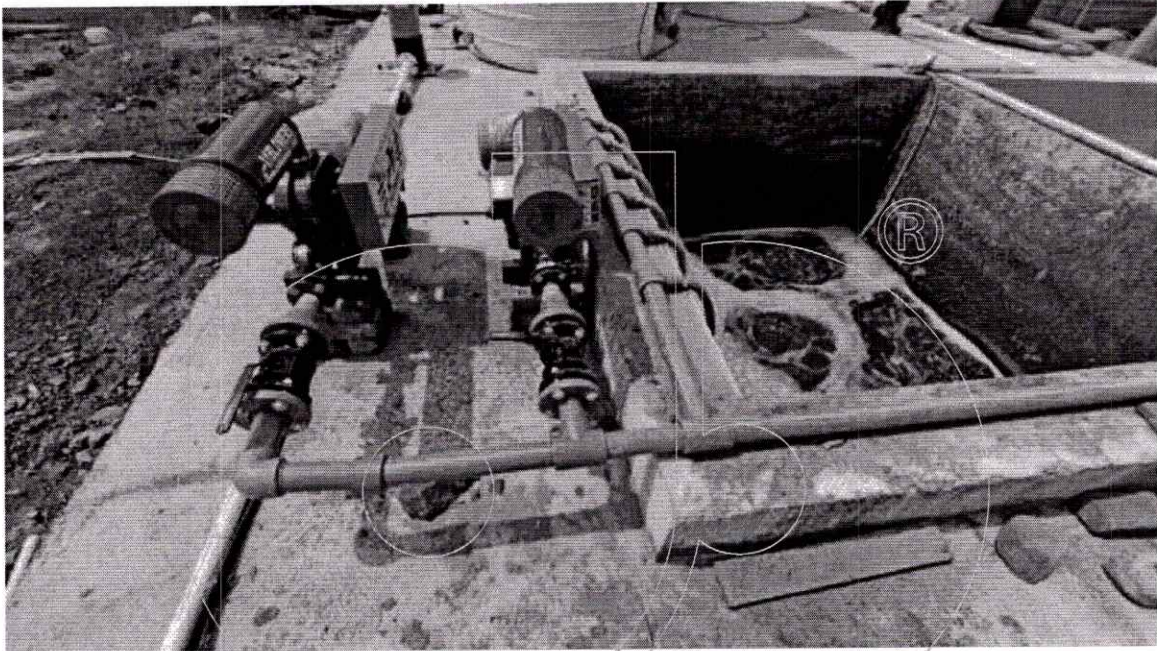
Blower for Aeration Tank with Diffuser
